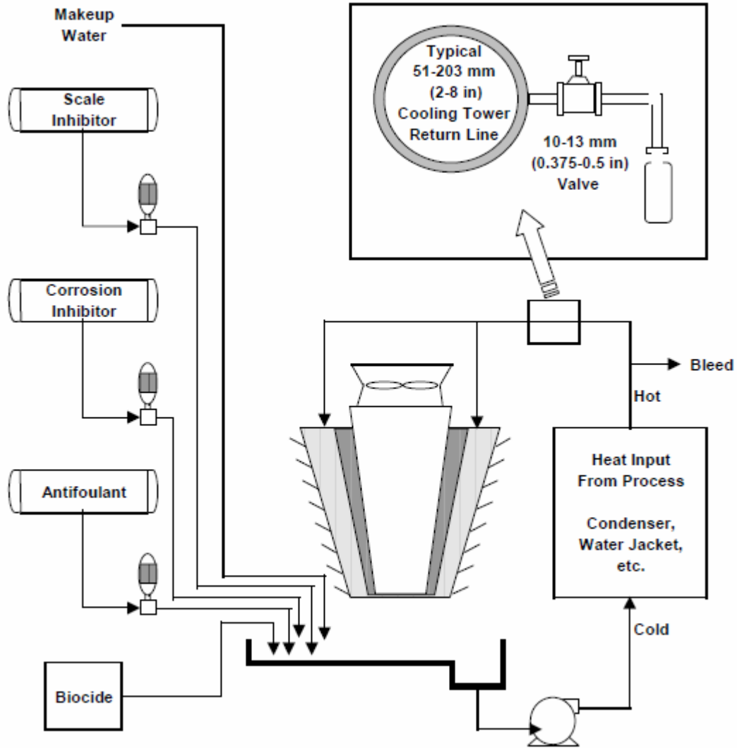
Figure 4 Typical Water Sampling Points for an Open Recirculating Cooling Water System
