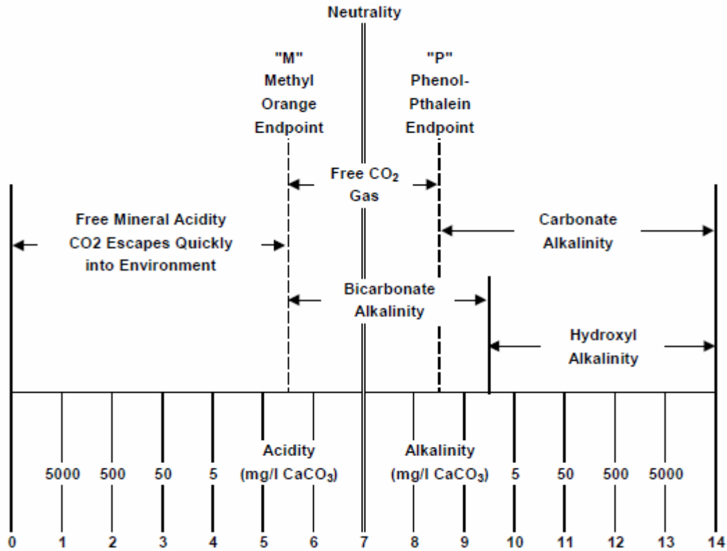
Figure 7 Acidity, Alkalinity, and pH Ranges
